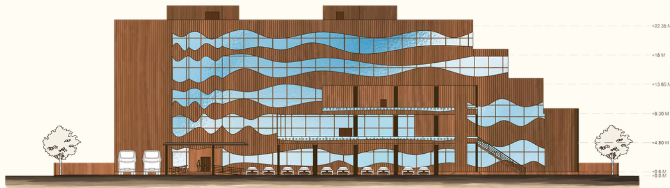
NORTH ELEVATION
